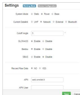
Figure 5.8 - Working mode and device configuration
